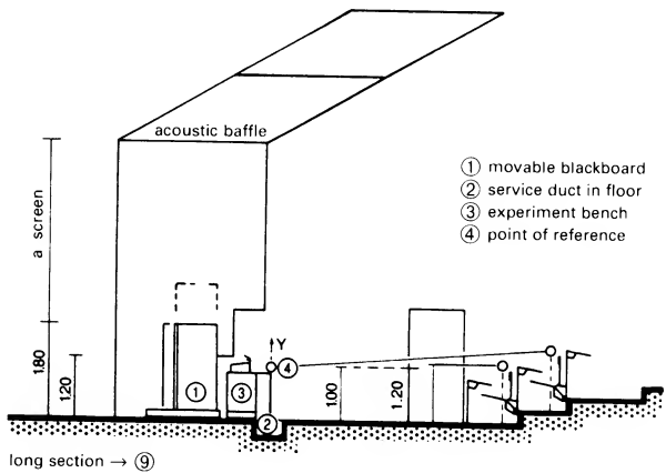
long section → ⑨
